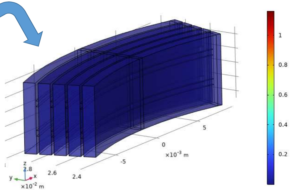
Time=0 s Volume: Magnetic flux density norm (T) Arrow Volume: Magnetic flux density
